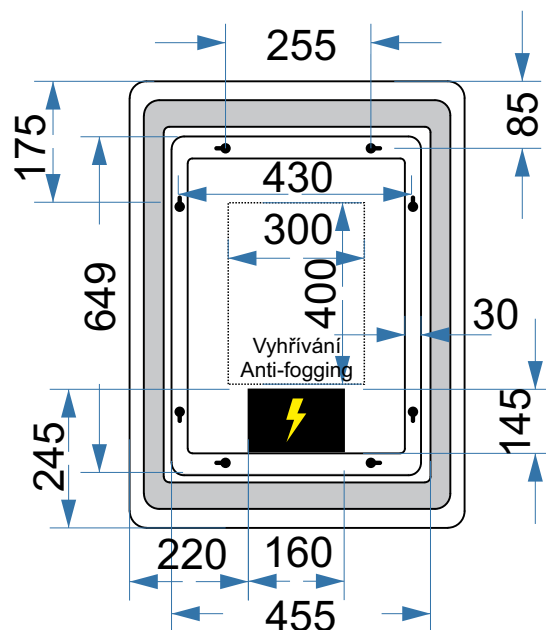
Pohled zezadu Rear view
