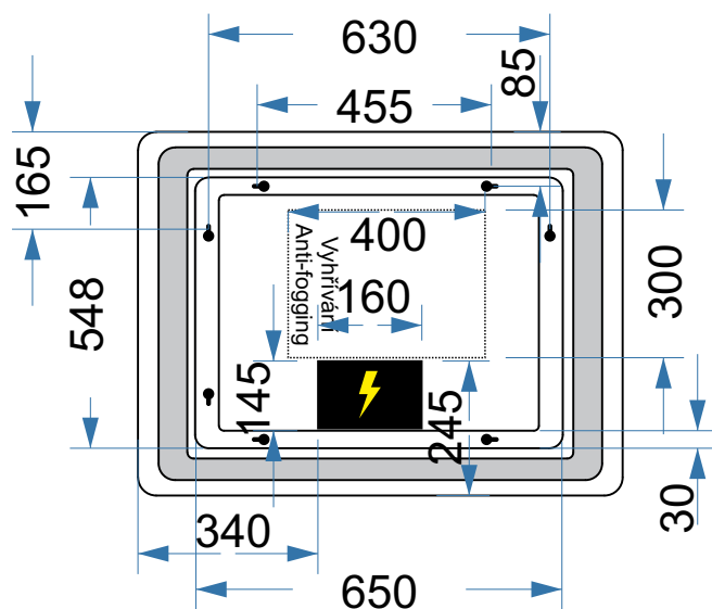
Pohled zezadu Rear view
